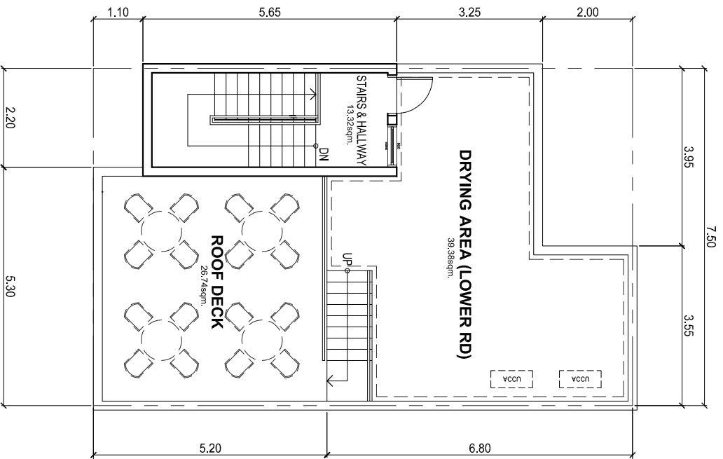
ROOF DECK PLAN
