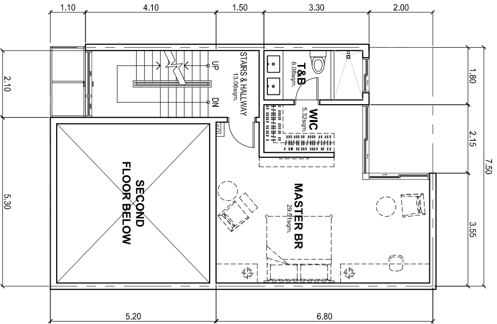
UPPER SECOND FLOOR PLAN
